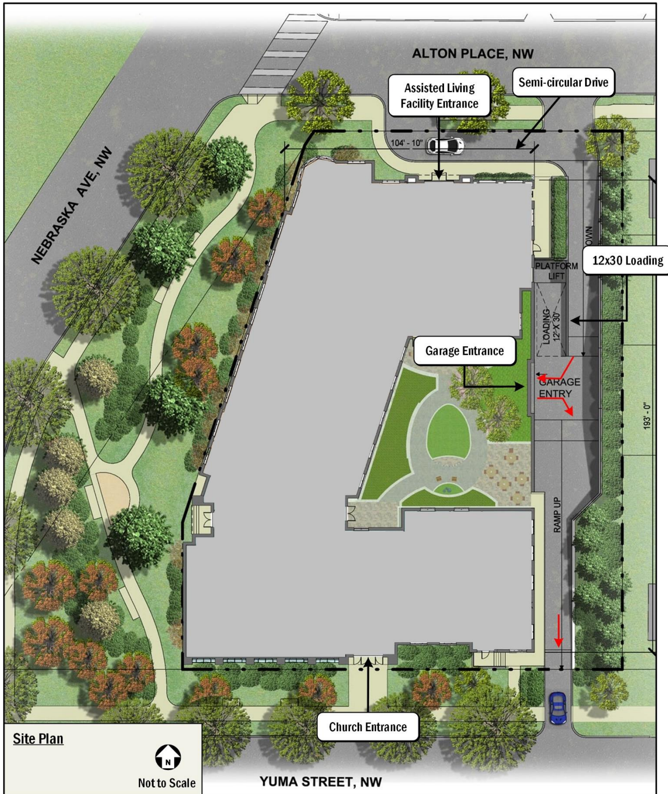
Figure 6: Site Plan
